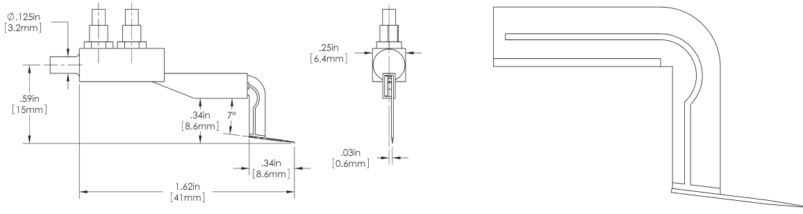
DCP-HTR Probe Body
