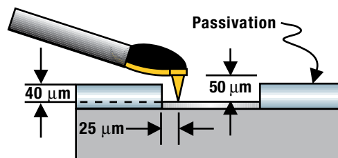
Figure 10: Maximum passivation thickness is 40 \mu\text{m} above the probe pad
