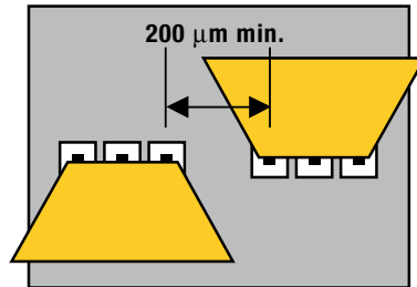
Figure 12: Rule 104 Minimum pad spacing with opposing, side-by-side probes is 200 μm.
