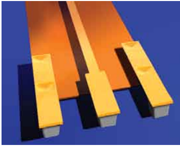
Figure 1: Infinity's microstrip transmission line construction reduces unwanted coupling
