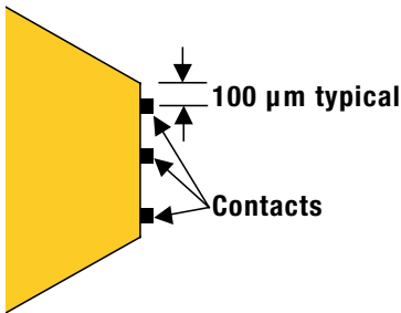
Figure 6: Substrate extension is typically 100 \mu\text{m}
