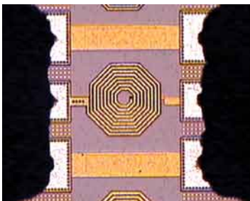
Figure 4: High frequency characterization of a spiral inductor
