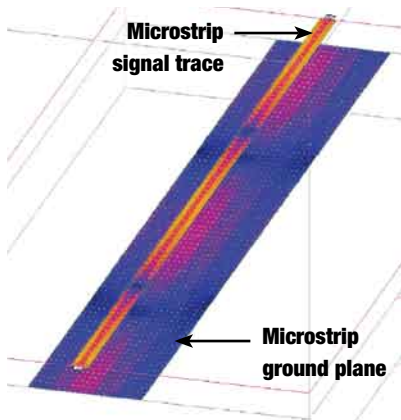
Figure 3 Traveling-wave voltage in microstrip
