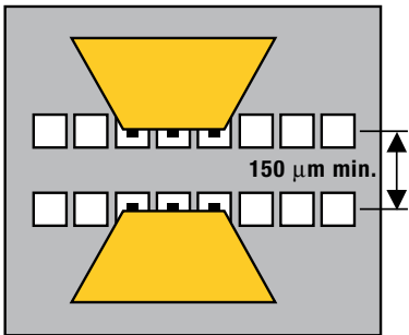
Figure 13: Rule 105 Minimum center-to-center pad spacing for parallel rows of pads with facing probes is 150 μm
