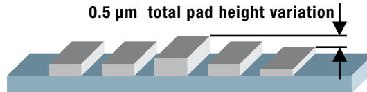
Figure 14: Rule 106 Maximum pad height variation in a row of pads contacted by one probe is 0.5 μm.
